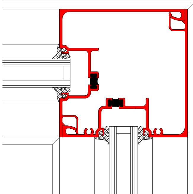
INSIDE CORNER
