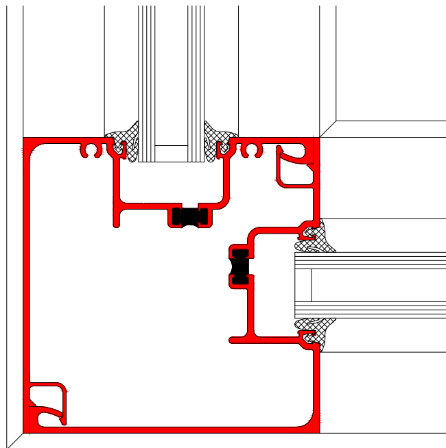
OUTSIDE CORNER
