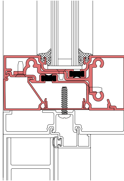
HEAD DETAIL
